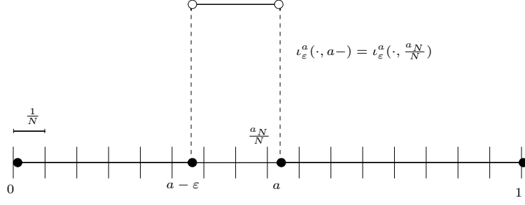
Figure 4.1: t_\varepsilon^a(\cdot, a^-) and t_\varepsilon^a(\cdot, \frac{a_N}{N})
