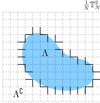
Figure 8.1: The darker region corresponds to \Lambda . The bolded bonds have exchanges rates \frac{|\vec{\zeta}_{x,j} \cdot e_j|}{N} , any other bond has exchange rate 1.
