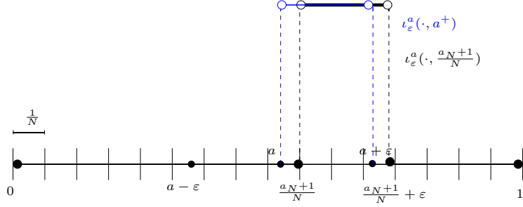
Figure 4.2: t_\varepsilon^a(\cdot, \frac{a_{N+1}}{N}) and t_\varepsilon^a(\cdot, a^+)
