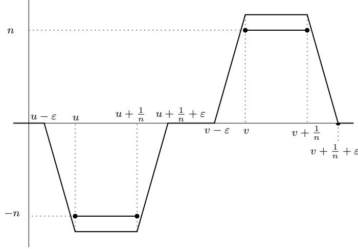
Figure A.1: Functions f_n^\varepsilon and f_n
