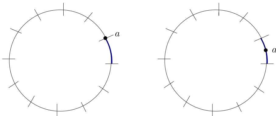
Figure 1: The slow bond is the bond associated with a .
