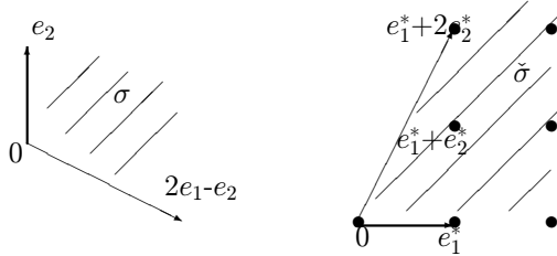
Fig. 6. A classical example.
