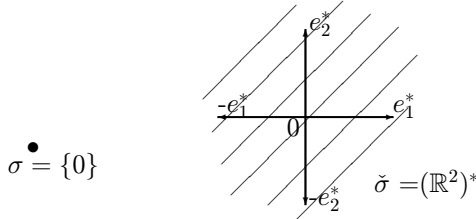
Fig. 5. The case \sigma = \{0\} .
