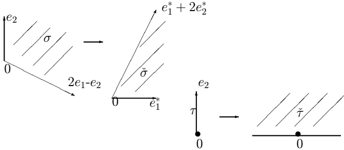
Fig. 2. Examples of dual cones
