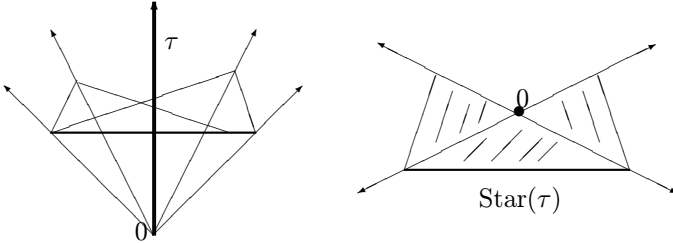
Fig. 19. Star of \tau
