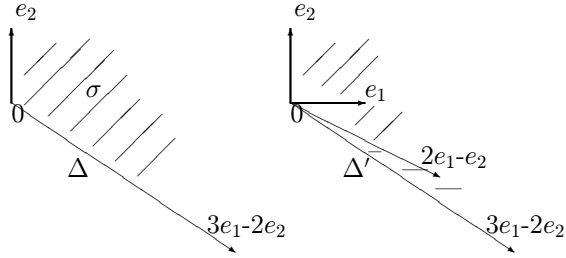
Fig. 31. Resolution of singularities.
