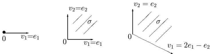
Fig. 1. Examples of cones
