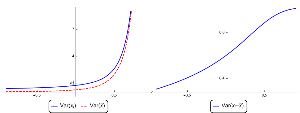
Figure 4: Effect of r on individual and aggregate volatility, and dispersion.
